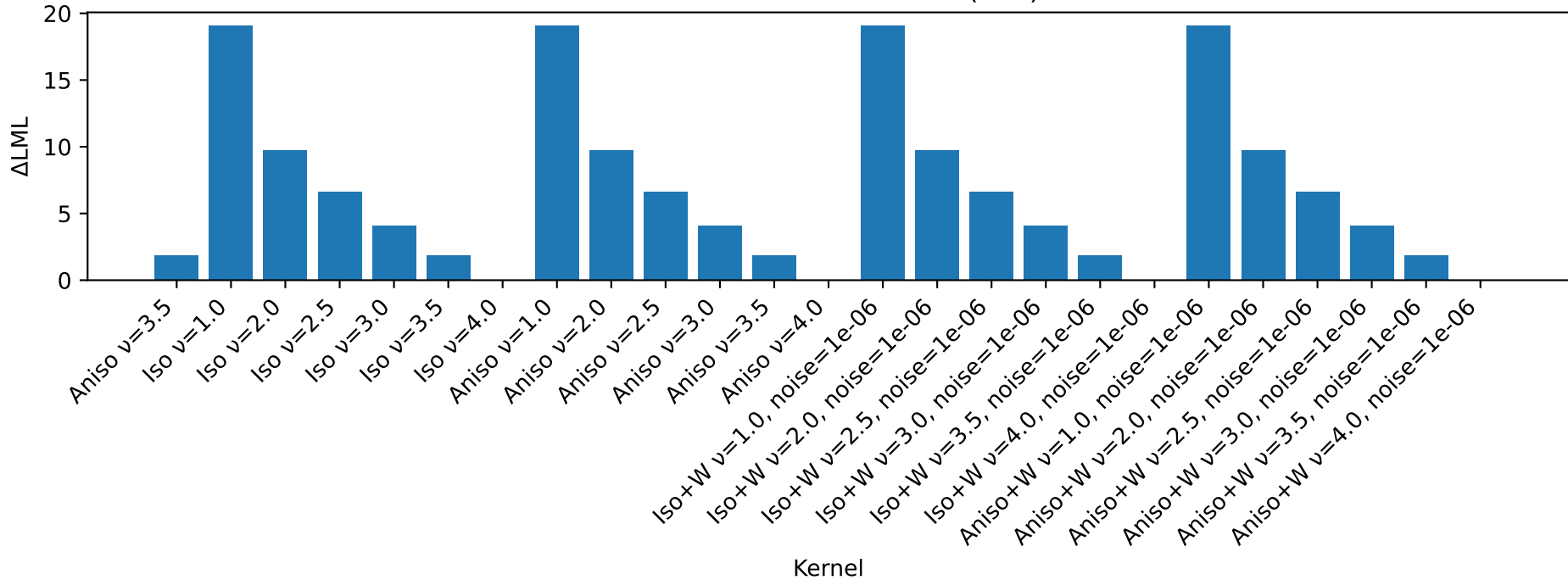
Difference from best LML (T15)
