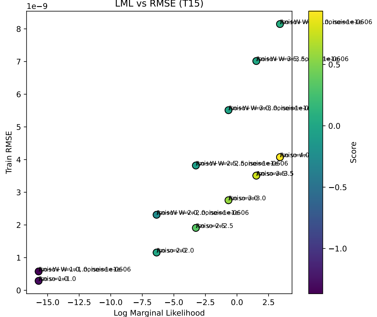
LML vs RMSE (T15)
