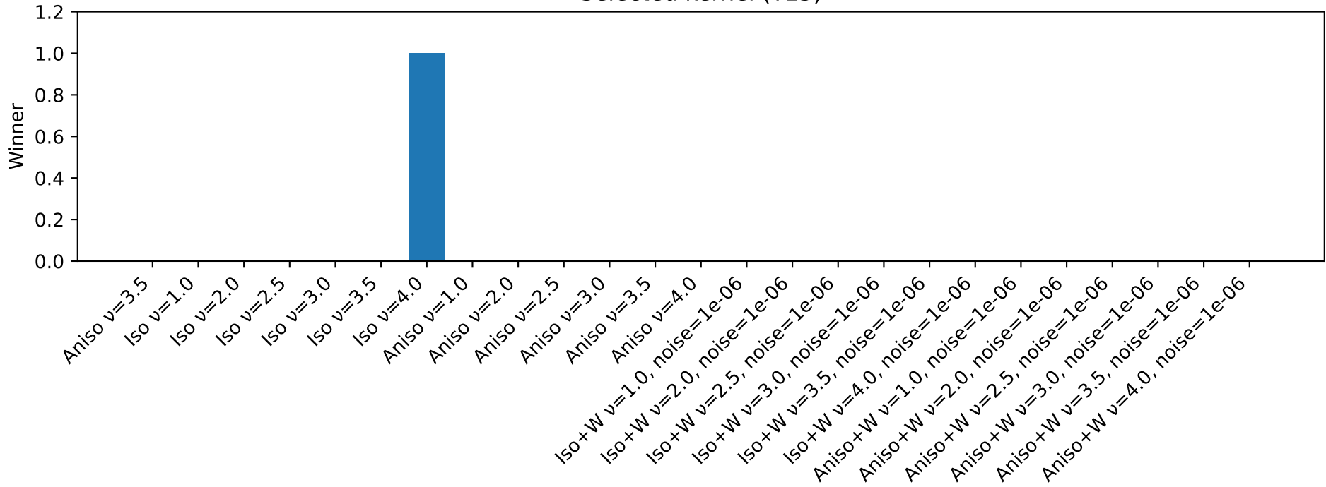
Selected kernel (T15)
