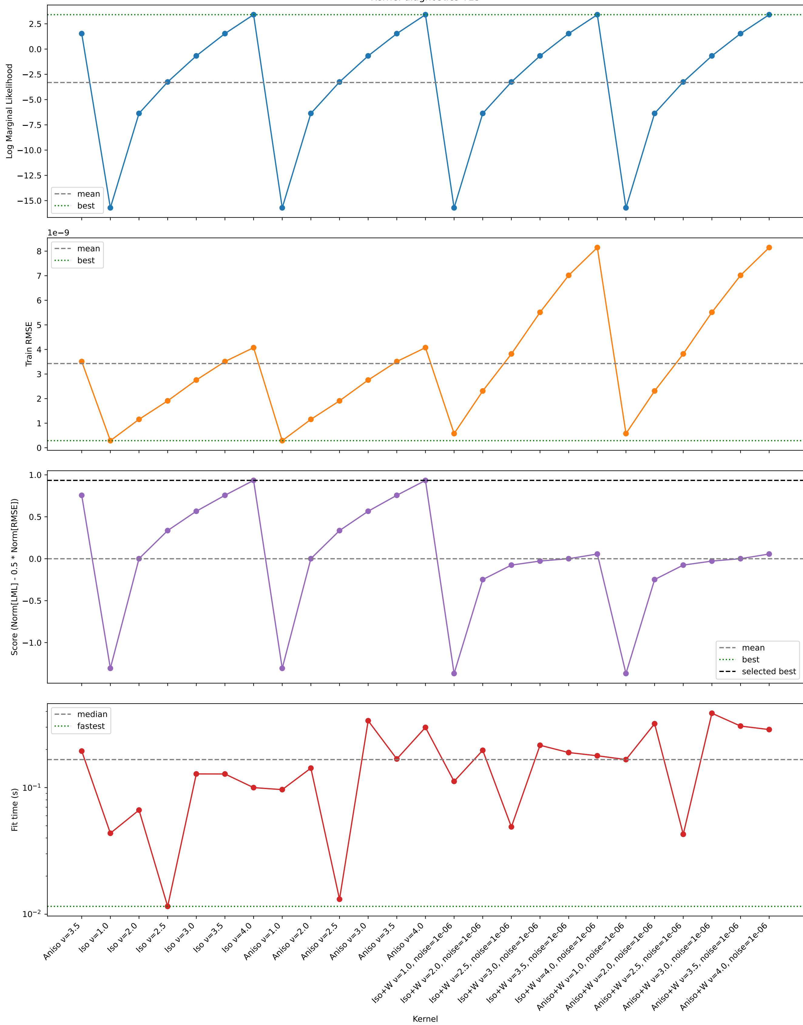
Kernel diagnostics T15
